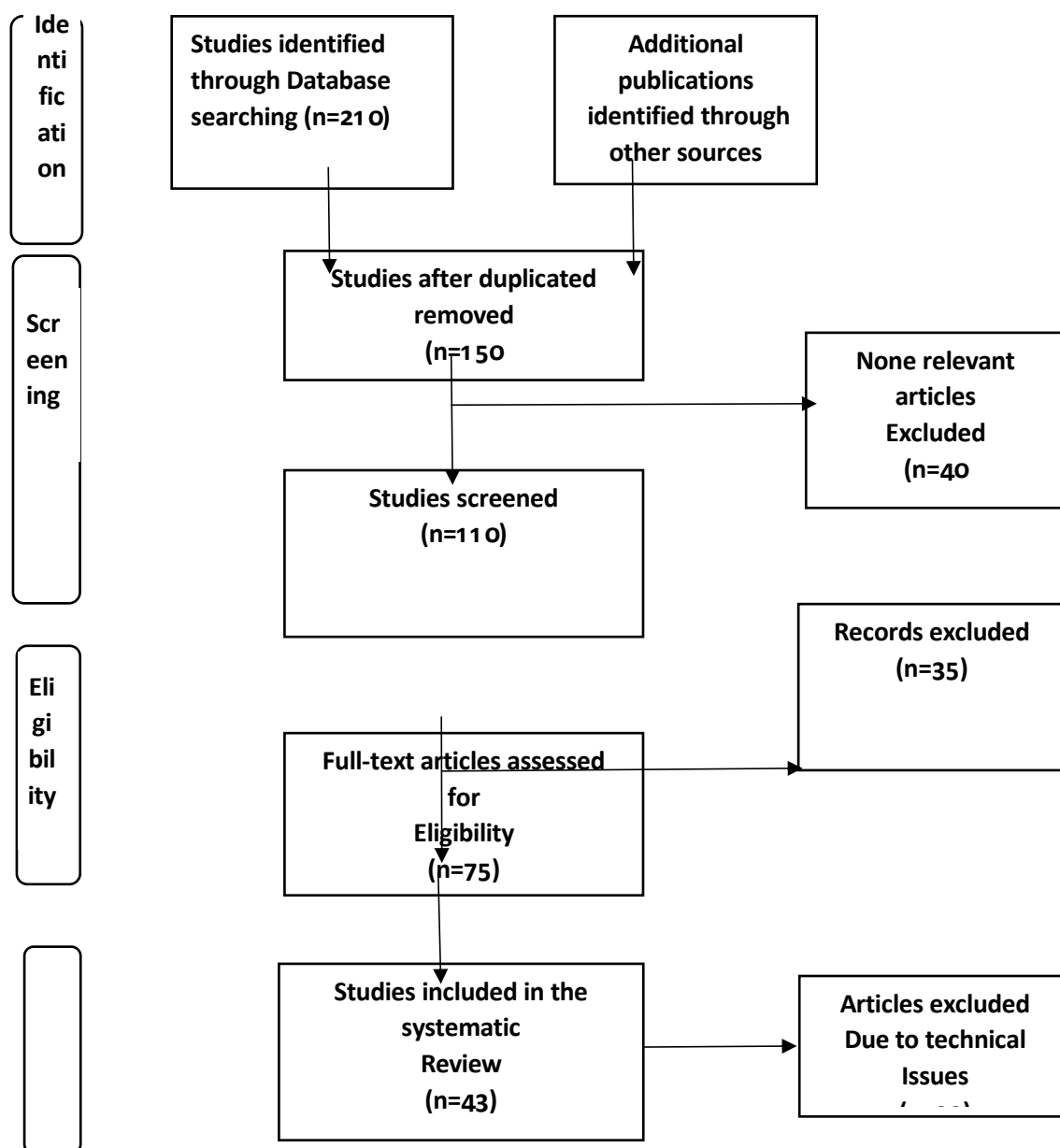
Figure 1: PRISMA Framework
